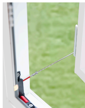
WOCD device is located on the interior of the sash and jamb.
